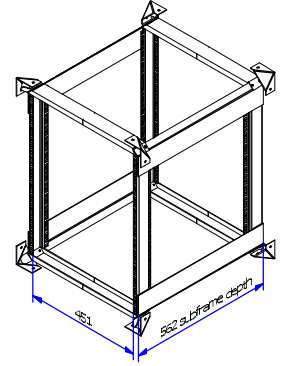
Subframe suspended with 8 x Anti-vibration Mounts (weight bearing 50kg, 90kg or 200kg)
