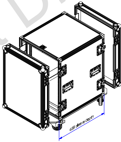
External Dimensions (excluding hardware) - 581W x 835D x 755H
