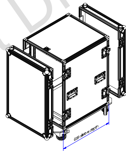
External Dimensions (excluding hardware) - 581W x 835D x 844H
