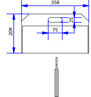
Moveable Partition
