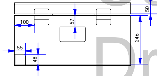
Base Plan
