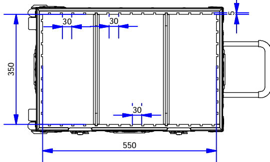
Base Plan
