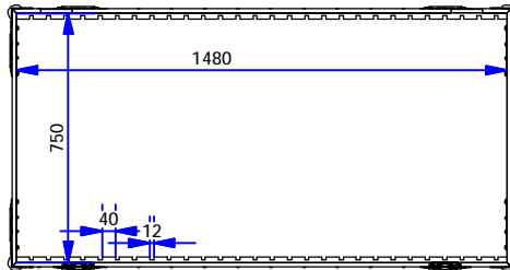
BASE VIEW
