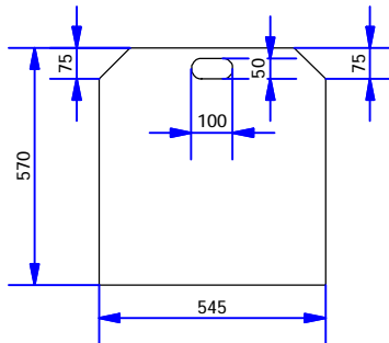
External Dimensions (excluding hardware); 976L x 586W x 603H
